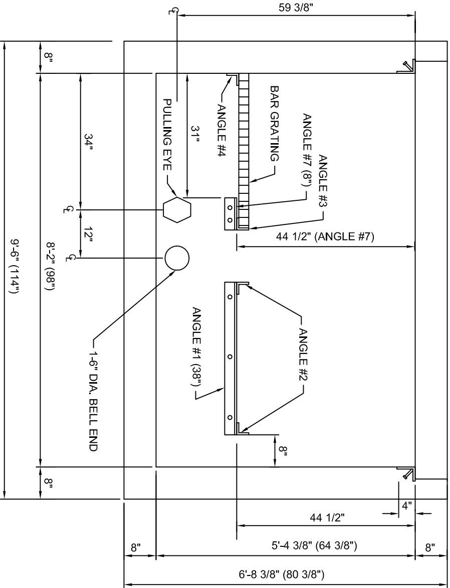
DETAIL SIDE "B" (STANDING INSIDE BOX)
