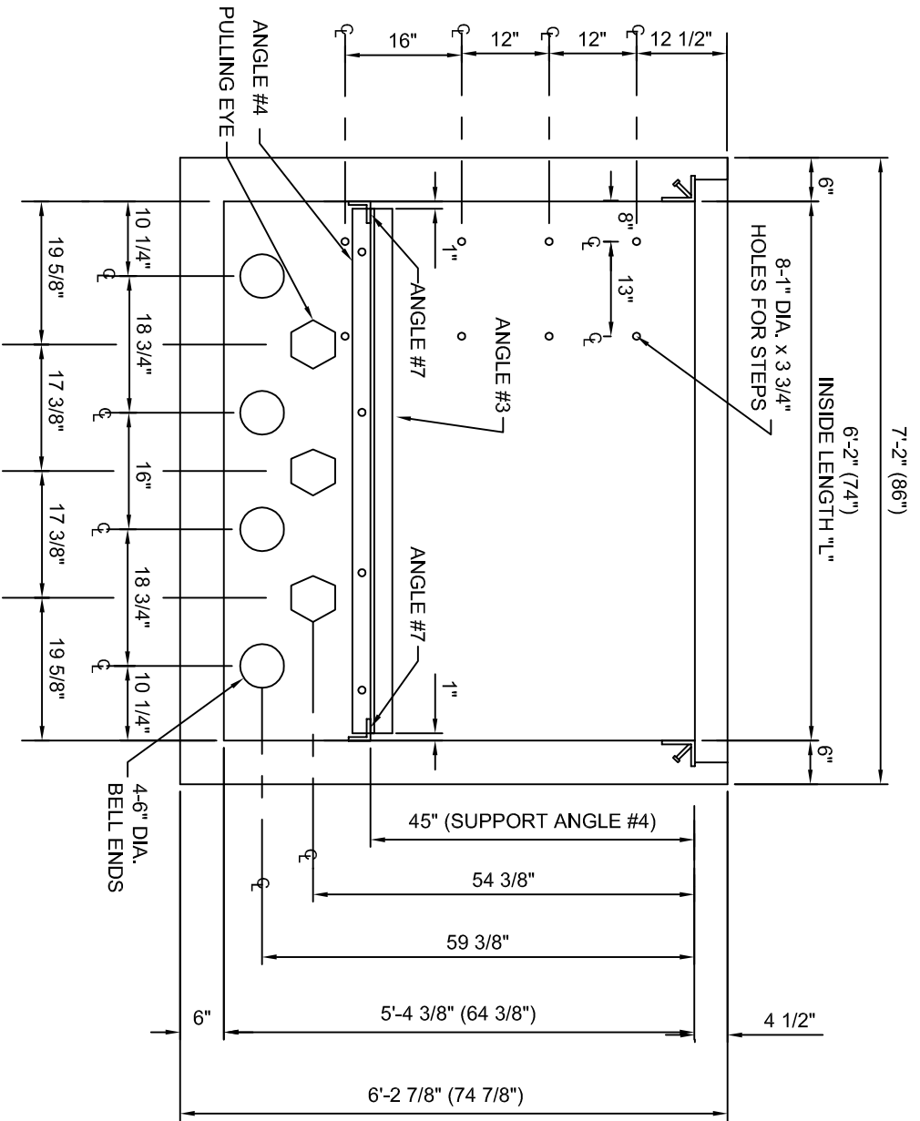
DETAIL SIDE "C"
