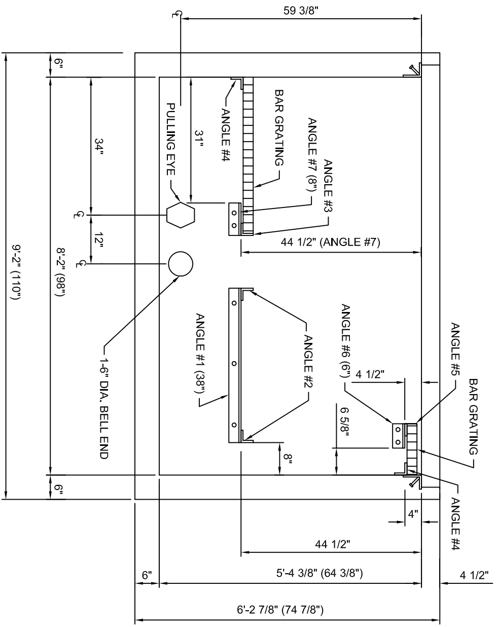
DETAIL SIDE "B" (STANDING INSIDE BOX)
