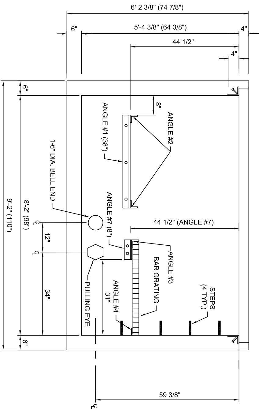
DETAIL SIDE "D" (STANDING INSIDE BOX)
