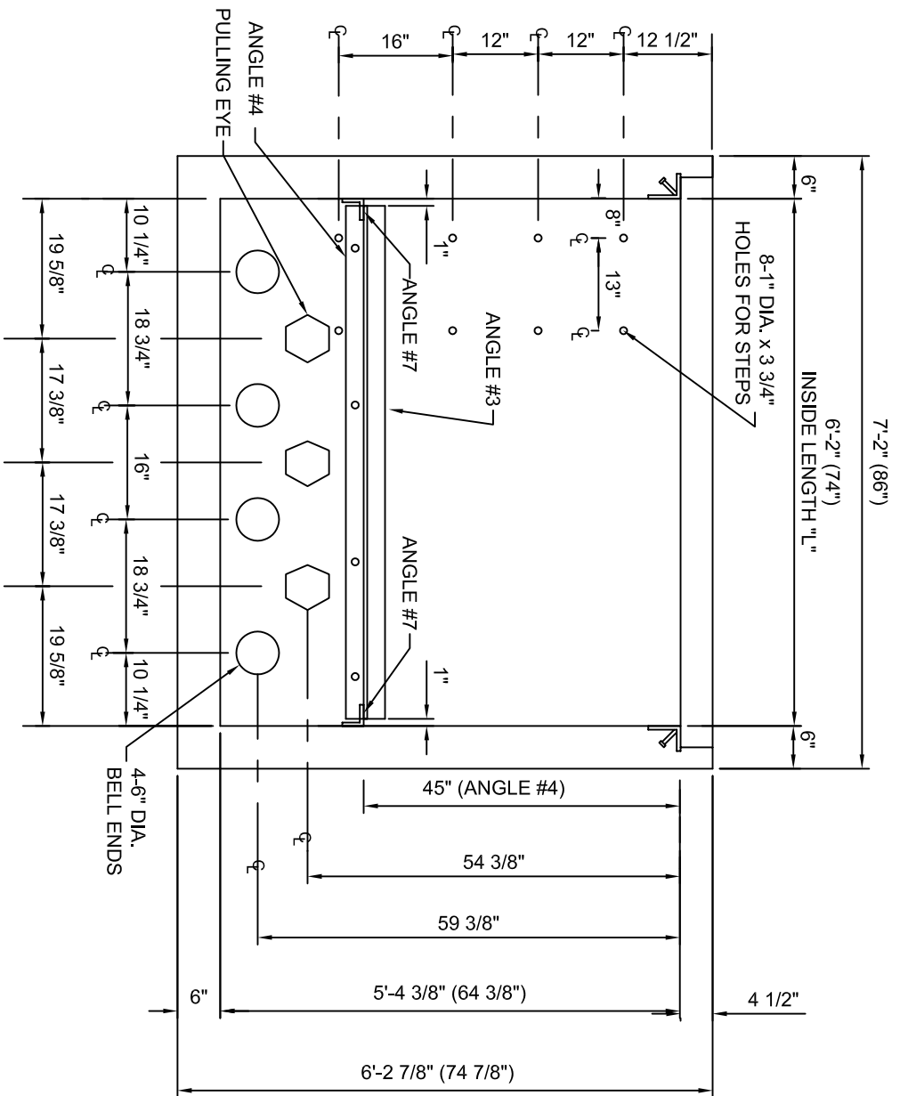
DETAIL SIDE "C" (STANDING INSIDE BOX)
