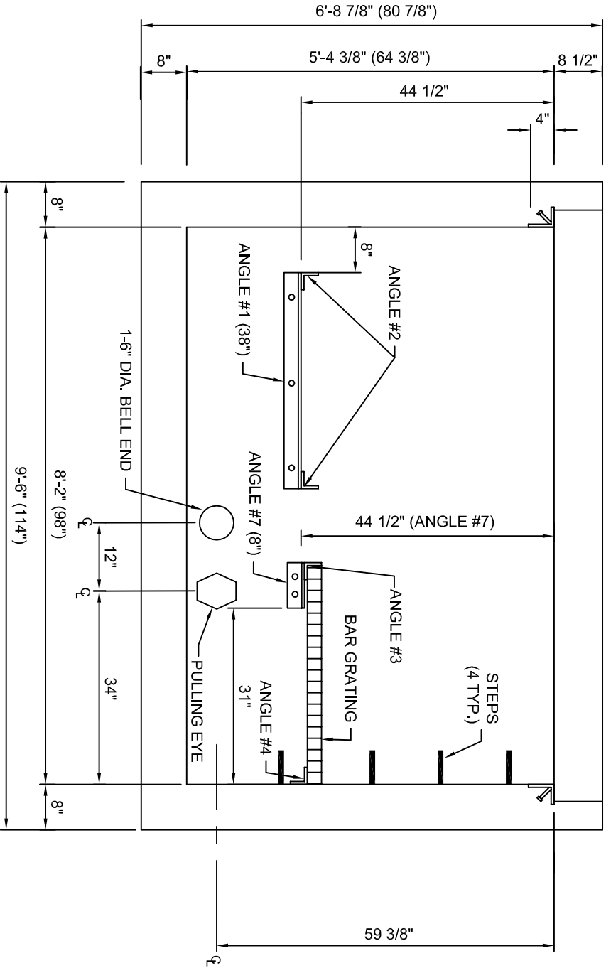
DETAIL SIDE "D" (STANDING INSIDE BOX)
