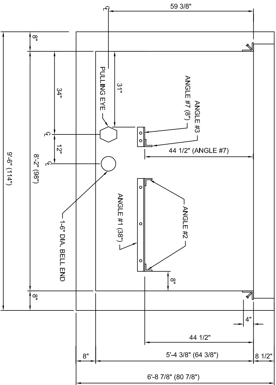
DETAIL SIDE "B" (STANDING INSIDE BOX)
