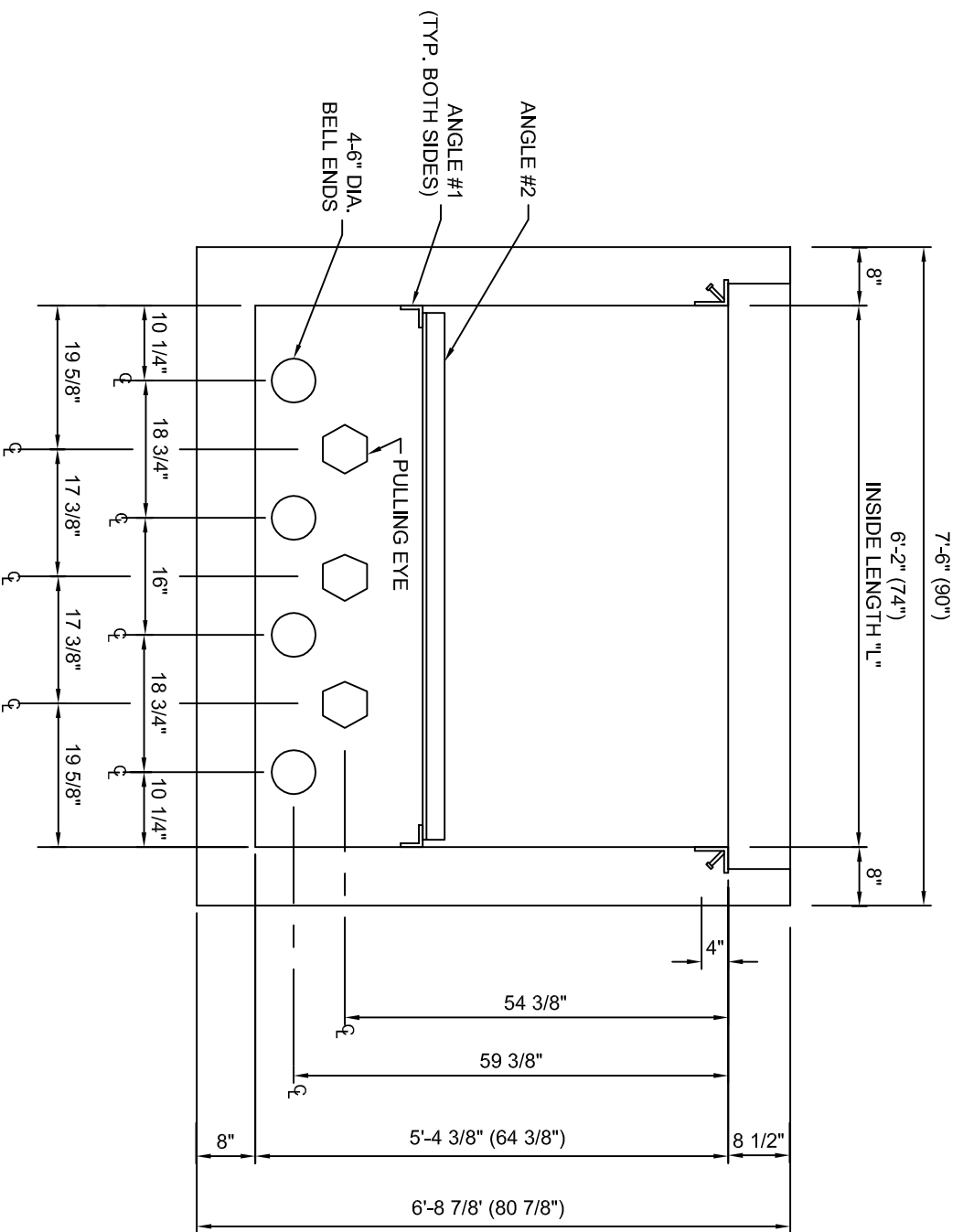
DETAIL SIDE "A" SWITCH GEAR END (STANDING INSIDE BOX)
