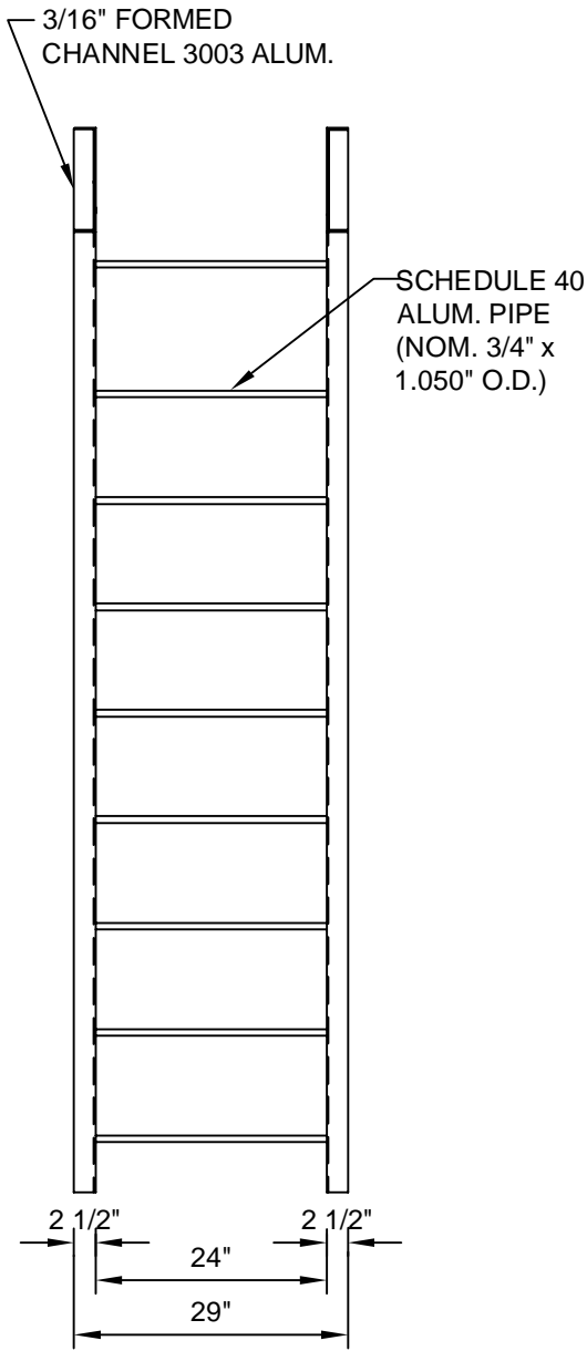
FRONT ELEVATION
