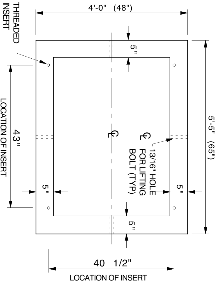
PLAN VIEW
