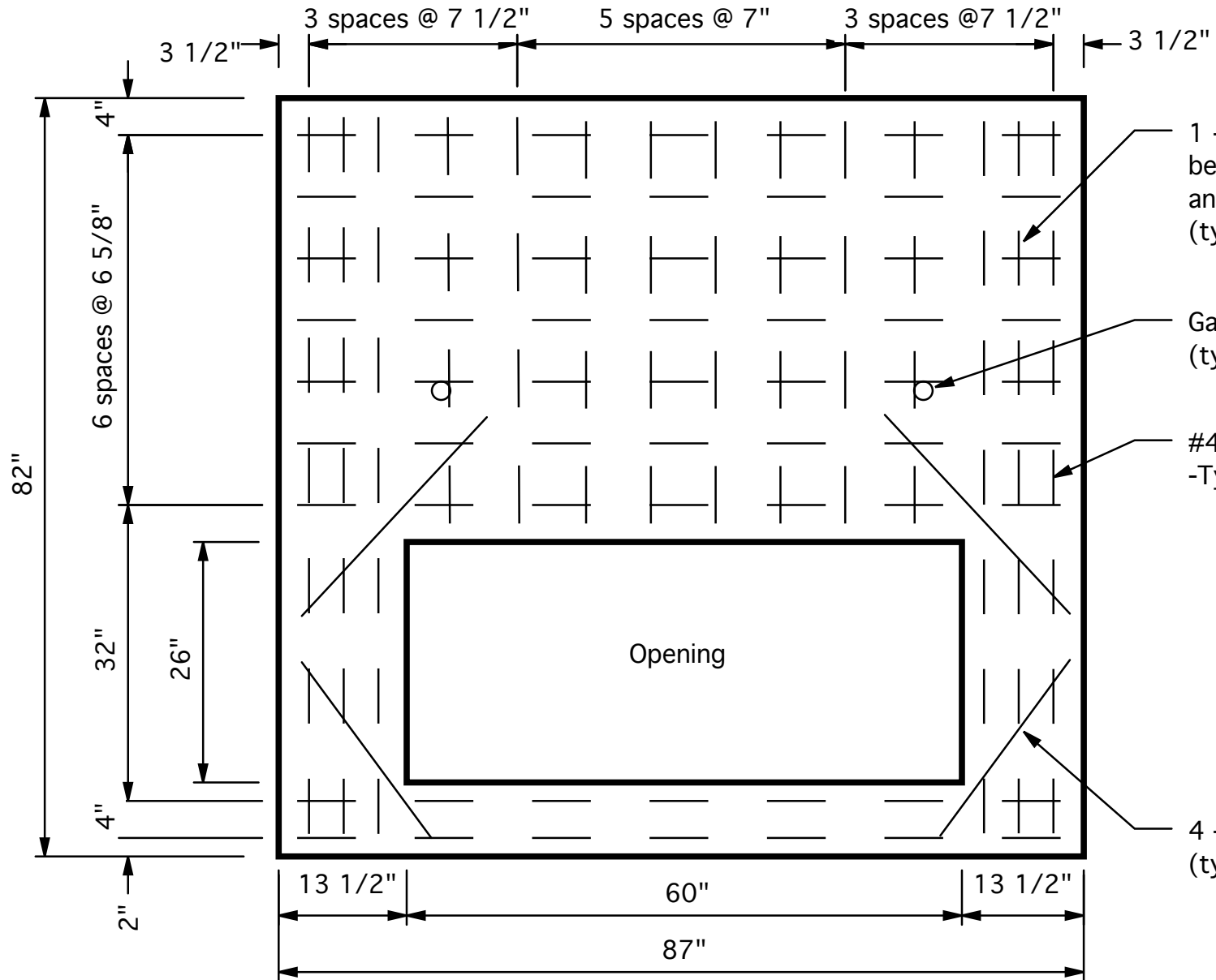
PLAN VIEW
